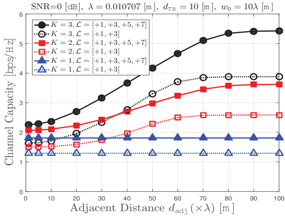
Fig. 6: Channel capacity with respect to the relative distance between adjacent transmit antennas.
